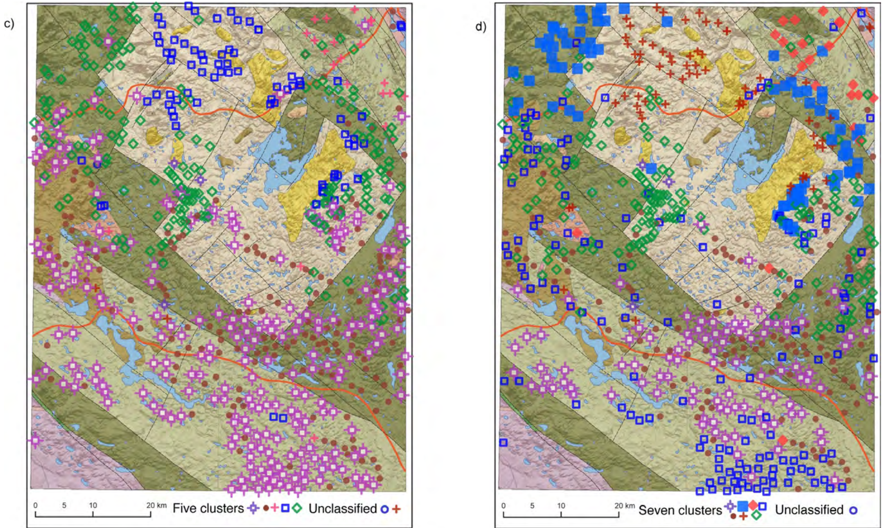
Figure 6 (continued). Results of cluster analysis of the clay fraction of till geochemical data (Mo, Cu, Pb, Zn, Ni, Co, Mn, Fe, As, U, Au, Sr, Cd, Sb, V, Th, Ca, La, Cr, Mg, Ba, Al, Na, K, Sc and Hg), central British Columbia. Samples were divided into c) five and d) seven clusters. Data are overlaid on the bedrock geology map presented in Figure 2. Note that although the number of clusters is set for each analysis, data that do not conform to a major cluster are assigned different symbols.
