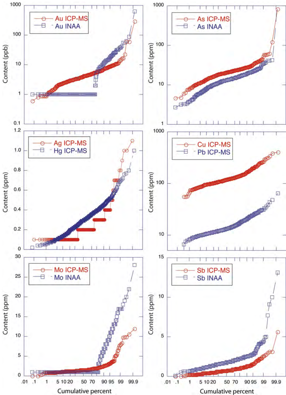
Figure 3a. Cumulative probability plots for Au, As, Ag, Hg, Cu, Pb, Mo and Sb, analyzed by aqua-regia digestion followed by inductively coupled plasma–mass spectrometry (ICP-MS) on the clay-sized fraction and/or instrumental neutron activation analysis (INAA) on the clay plus silt-sized fraction. Anomalous metal concentrations typically occur around the 90 to 95th percentiles, where there is a change in slope on the probability plot.
