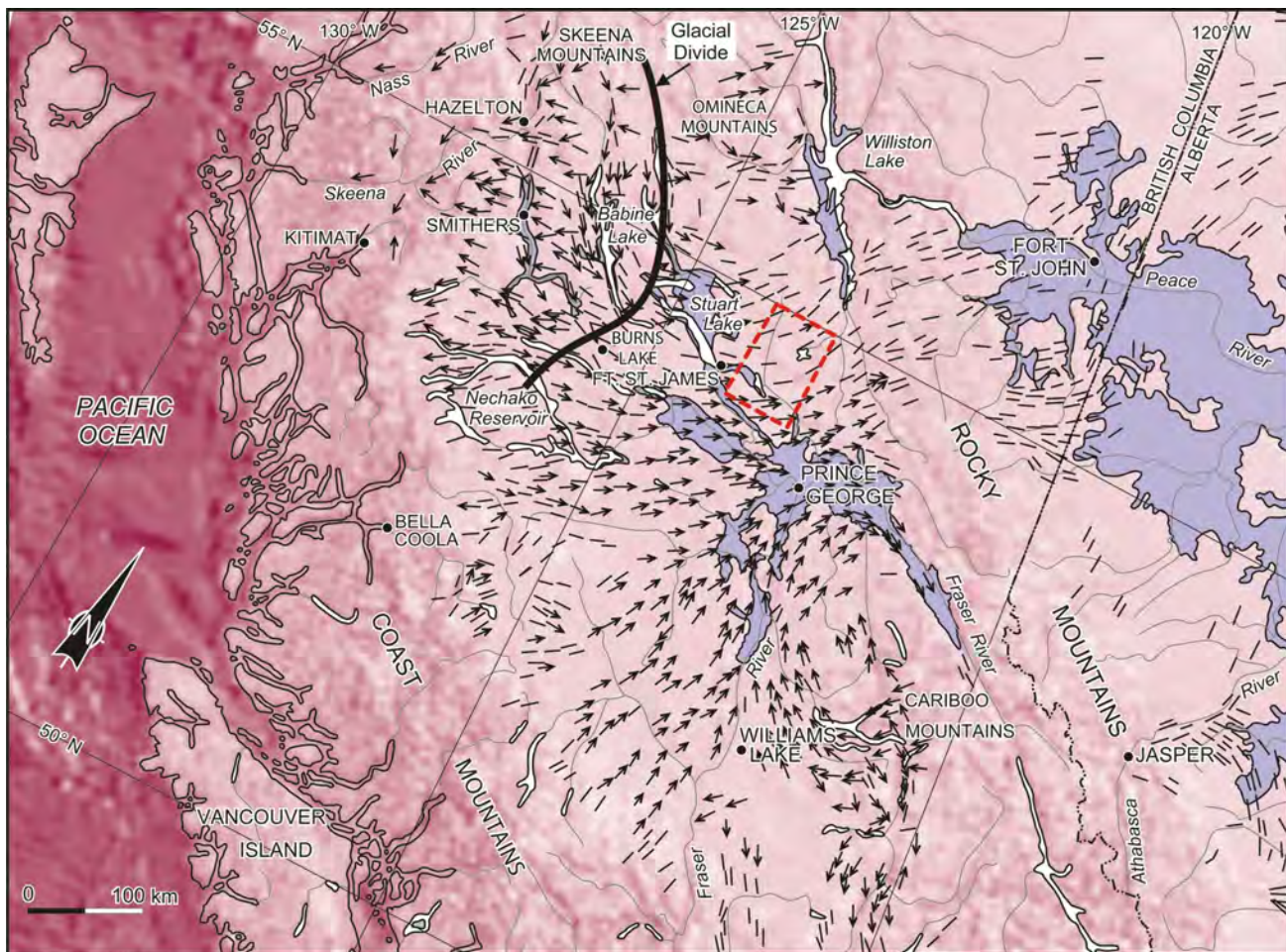
Figure 1. Northern British Columbia with dominant ice-flow directions (shown by the black arrows and short black lines) for the Late Wisconsinan Fraser glaciation (modified from Stumpf et al., 2000). Light blue areas indicate the approximate distribution of deglacial lake sediments, which can be a hindrance to drift prospecting. Red dashed line delineates the study area, which is shown in detail in Figure 2.
