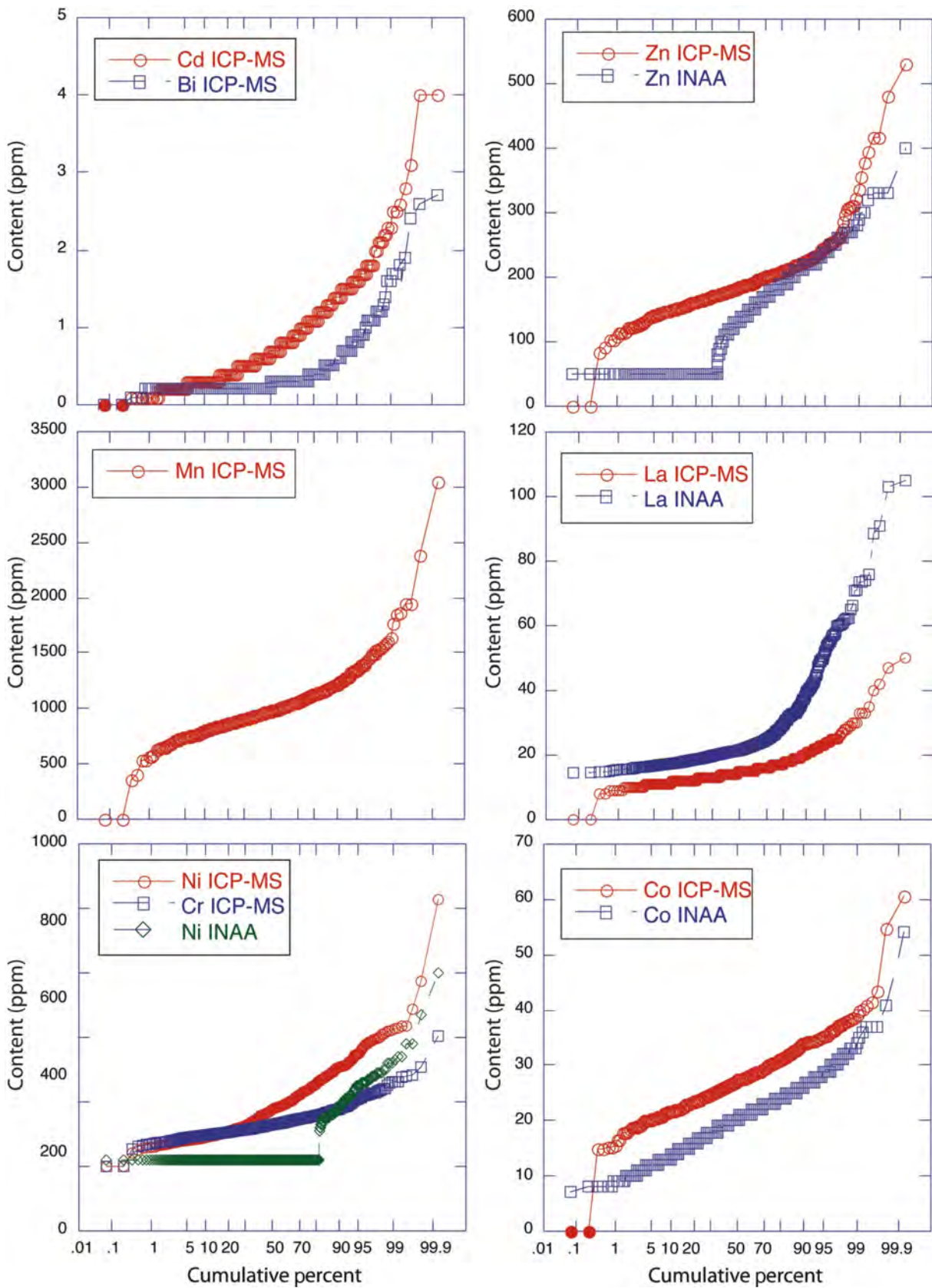
Figure 3b. Cumulative probability plots for Cd, Bi, Zn, Mn, La, Ni, Cr and Co, analyzed by aqua-regia digestion followed by inductively coupled plasma–mass spectrometry (ICP-MS) on the clay-sized fraction and/or instrumental neutron activation analysis (INAA) on the clay plus silt-sized fraction. Anomalous metal concentrations typically occur around the 90 to 95th percentiles, where there is a change in slope on the probability plot.
