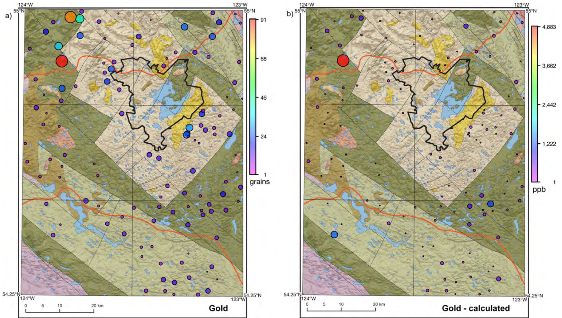
Figure 5. Proportional dot maps for a) gold grain counts from heavy mineral concentrates from 10 kg till samples, central British Columbia. Also presented are b) calculated gold contents (ppb) of heavy mineral concentrates, which are based on gold grain counts. Data are overlaid on the bedrock geology map presented in Figure 2.
