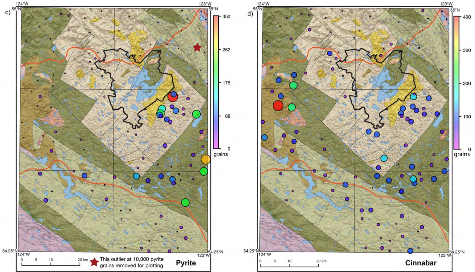
Figure 5 (continued). Proportional dot maps for c) pyrite and d) cinnabar grain counts from heavy mineral concentrates from 10 kg till samples, central British Columbia. Data are overlaid on the bedrock geology map presented in Figure 2.
