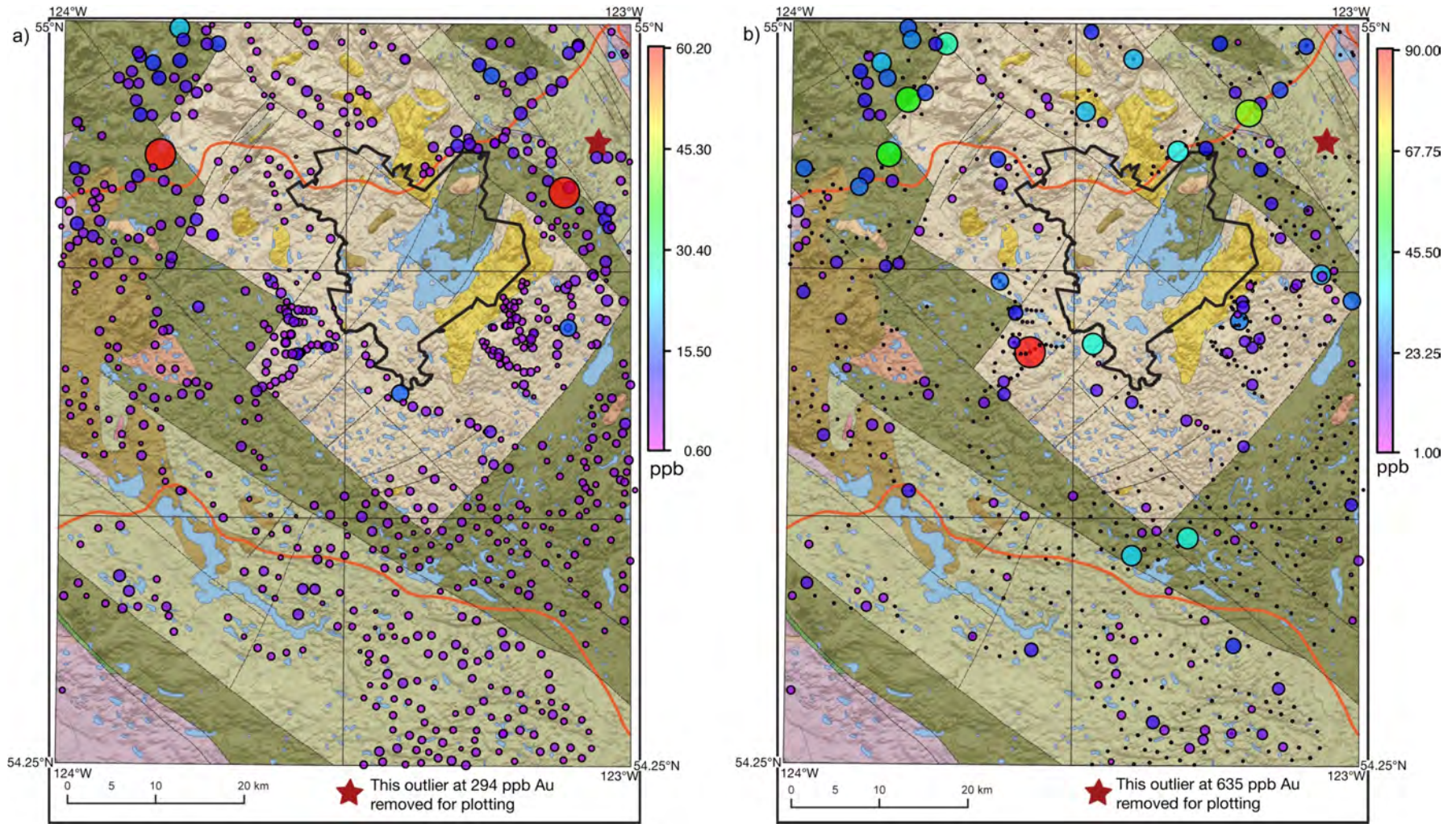
Figure 4. Proportional dot maps of selected elements from till geochemical analyses, central British Columbia: a) Au contents (clay-sized fraction) by inductively coupled plasma–mass spectrometry (ICP-MS) and b) Au contents (clay plus silt-sized fraction) by instrumental neutron activation analysis (INAA). Size of dots are proportional to the content. Data are overlaid on the bedrock geology map presented in Figure 2.
