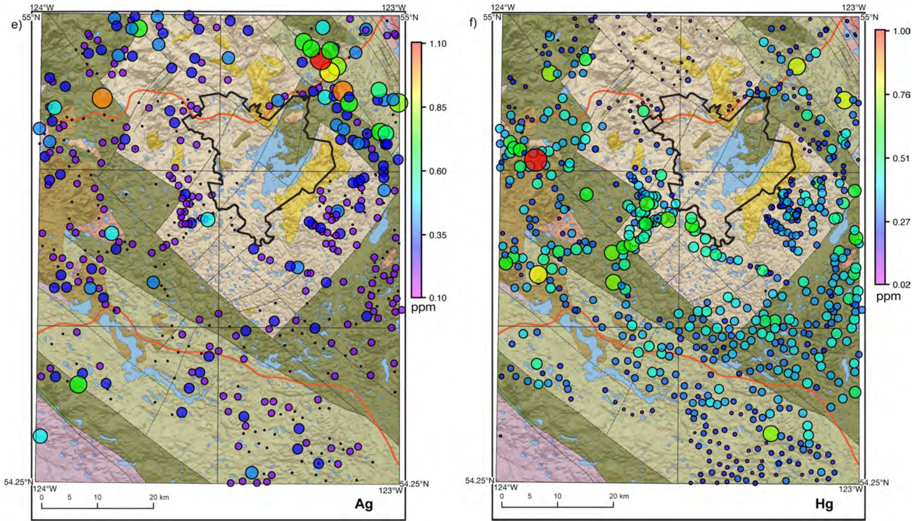
Figure 4 (continued). Proportional dot maps of selected elements from till geochemical analyses, central British Columbia: e) Ag contents (clay-sized fraction) by ICP-MS and f) Hg contents (clay-sized fraction) by ICP-MS. Size of dots are proportional to the content. Data are overlaid on the bedrock geology map presented in Figure 2.
