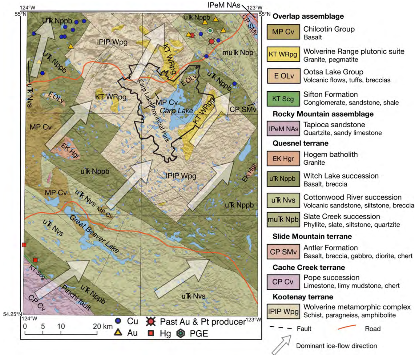
Figure 2. Major bedrock geological units of the study area, central British Columbia (modified from Struik, 1994 and Logan et al., 2010). Also shown are mineral occurrences for different commodity types (after BC Geological Survey, 2010) and the dominant ice-flow direction (light-coloured arrows; after Sacco et al., 2010).
