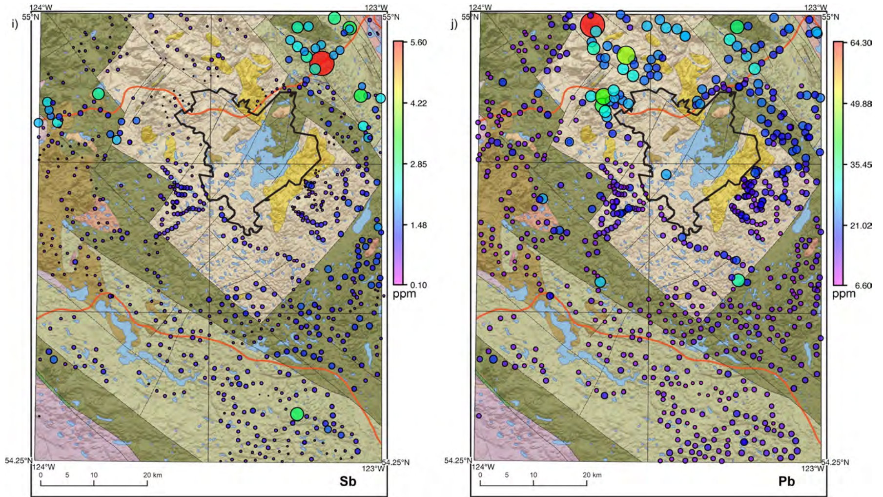
Figure 4 (continued). Proportional dot maps of selected elements from till geochemical analyses, central British Columbia: i) Sb contents (clay-sized fraction) by ICP-MS and j) Pb contents (clay-sized fraction) by ICP-MS. Size of dots are proportional to the content. Data are overlaid on the bedrock geology map presented in Figure 2.
