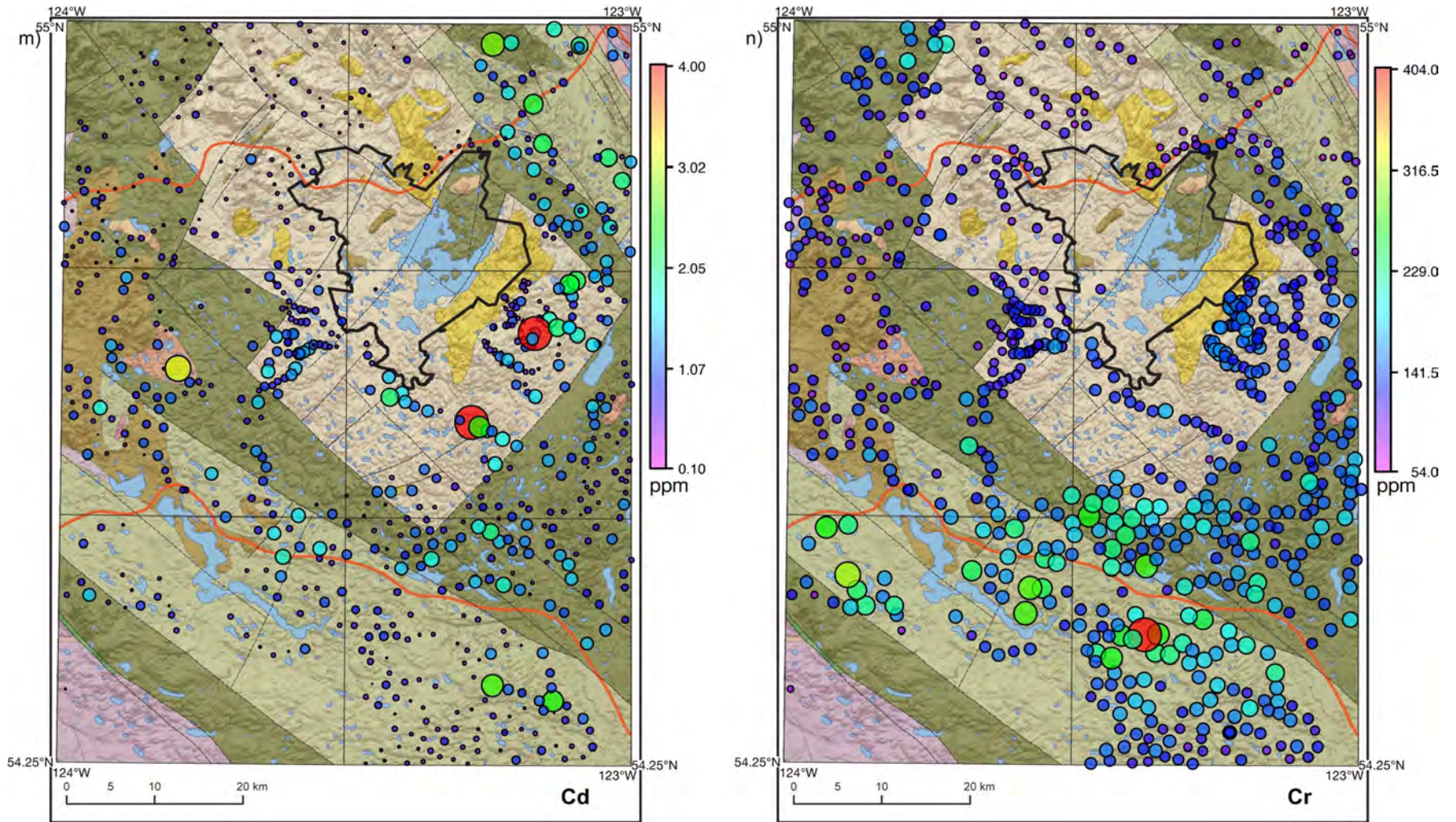
Figure 4 (continued). Proportional dot maps of selected elements from till geochemical analyses, central British Columbia: m) Cd contents (clay-sized fraction) by ICP-MS and n) Cr contents (clay-sized fraction) by ICP-MS. Size of dots are proportional to the content. Data are overlaid on the bedrock geology map presented in Figure 2.
