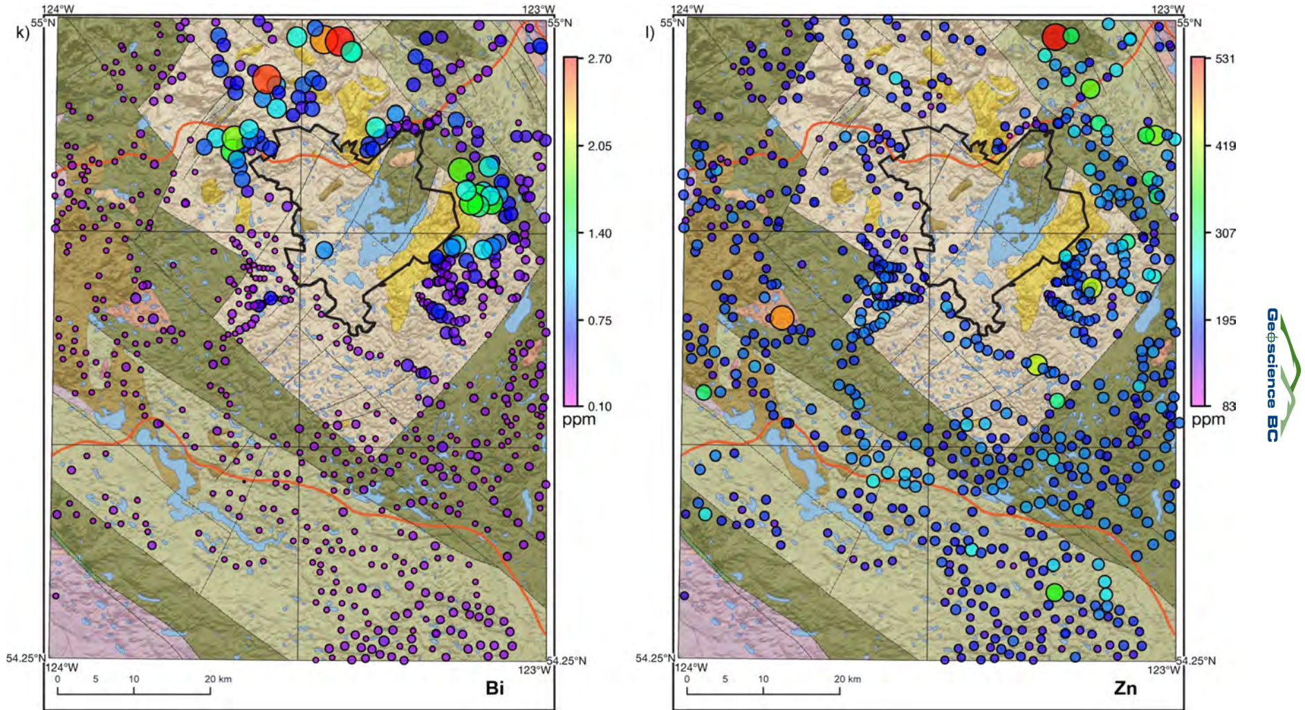
Figure 4 (continued). Proportional dot maps of selected elements from till geochemical analyses, central British Columbia: k) Bi contents (clay-sized fraction) by ICP-MS and l) Zn contents (clay-sized fraction) by ICP-MS. Size of dots are proportional to the content. Data are overlaid on the bedrock geology map presented in Figure 2.
