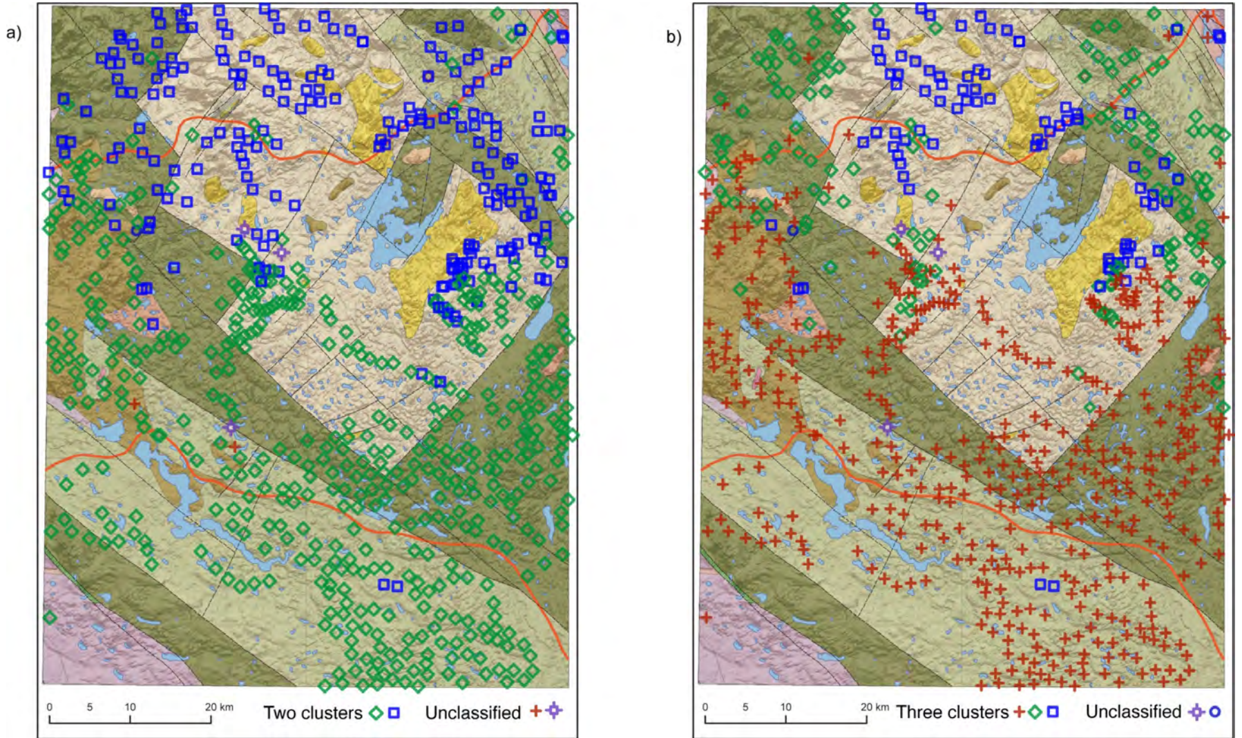
Figure 6. Results of cluster analysis of the clay fraction of till geochemical data (Mo, Cu, Pb, Zn, Ni, Co, Mn, Fe, As, U, Au, Sr, Cd, Sb, V, Th, Ca, La, Cr, Mg, Ba, Al, Na, K, Sc and Hg), central British Columbia. Samples were divided into a) two and b) three clusters. Data are overlaid on the bedrock geology map presented in Figure 2. Note that although the number of clusters is set for each analysis, data that do not conform to a major cluster are assigned different symbols.
