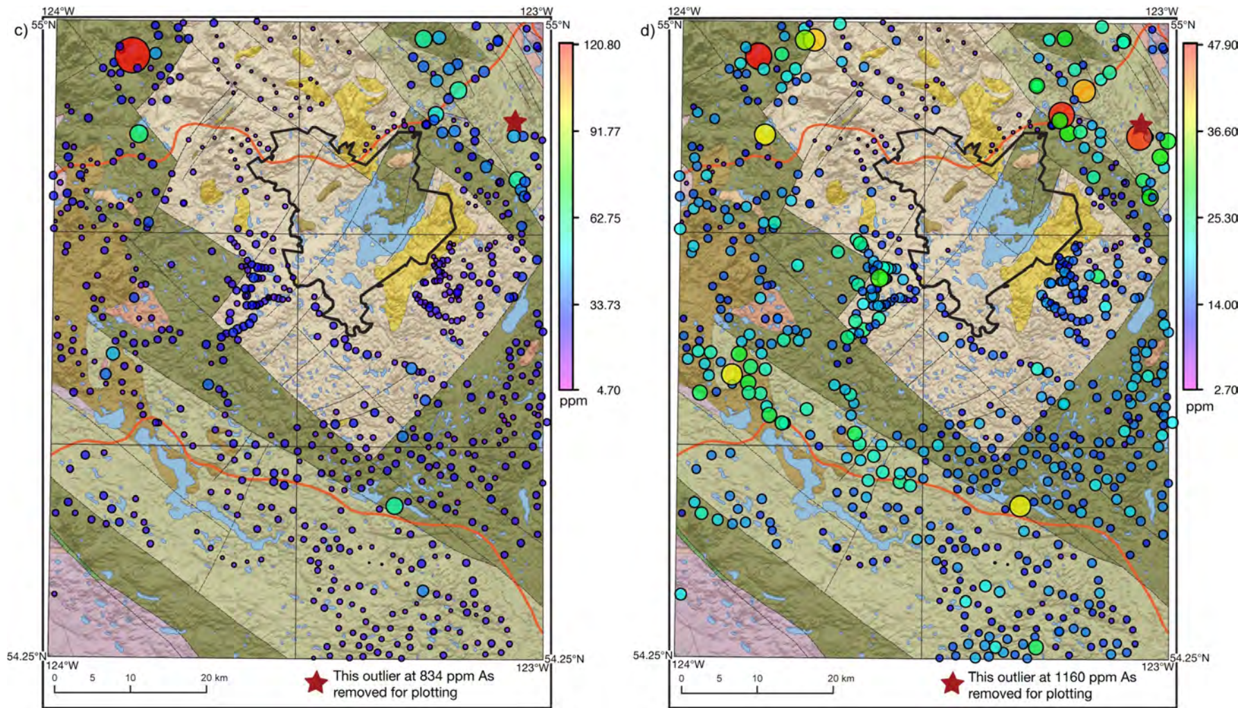
Figure 4 (continued). Proportional dot maps of selected elements from till geochemical analyses, central British Columbia: c) As contents (clay-sized fraction) by ICP-MS and d) As contents (clay plus silt-sized fraction) by INAA. Size of dots are proportional to the content. Data are overlaid on the bedrock geology map presented in Figure 2.
