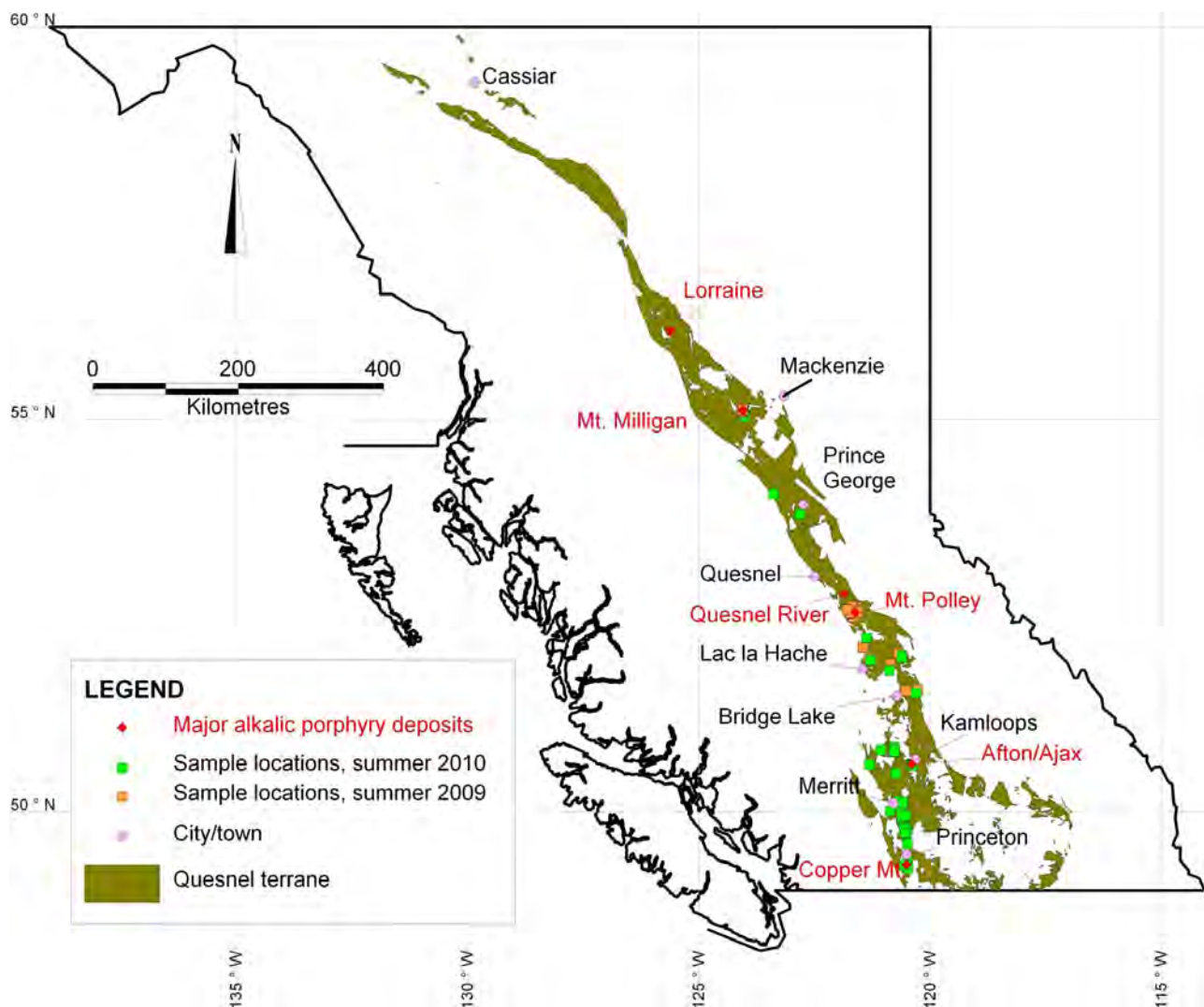
Figure 1. Major alkali porphyry Cu-Au deposits in the Quesnel terrane of British Columbia, showing sample locations from 2009 and 2010 fieldwork.
