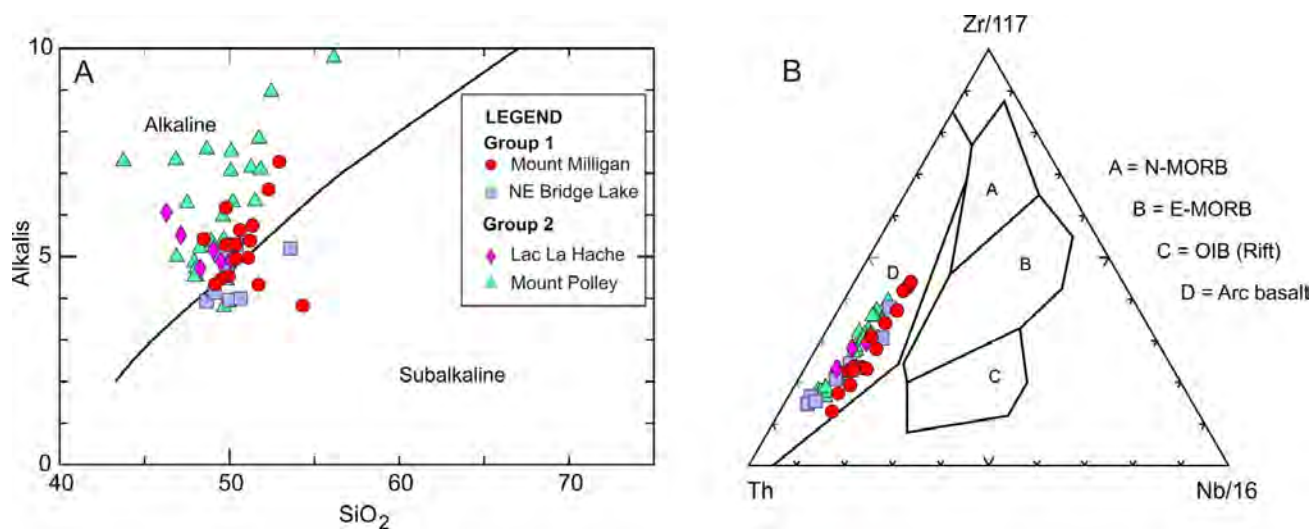
Figure 3. Classification of Nicola Group basalts: A) Plot of SiO 2 vs. Na 2 O+K 2 O (Irvine and Baragar, 1971), indicating the alkaline nature of the basalts of the Quesnel terrane; rocks from northeastern Bridge Lake and some from Mount Milligan have a subalkaline signature (Group 1), whereas basalts from Mount Polley and Lac la Hache are somewhat more alkaline (Group 2); B) Th–Zr/117–Nb/16 plot (Wood, 1980), indicating that all the rocks belong to a magmatic-arc tectonic setting.
