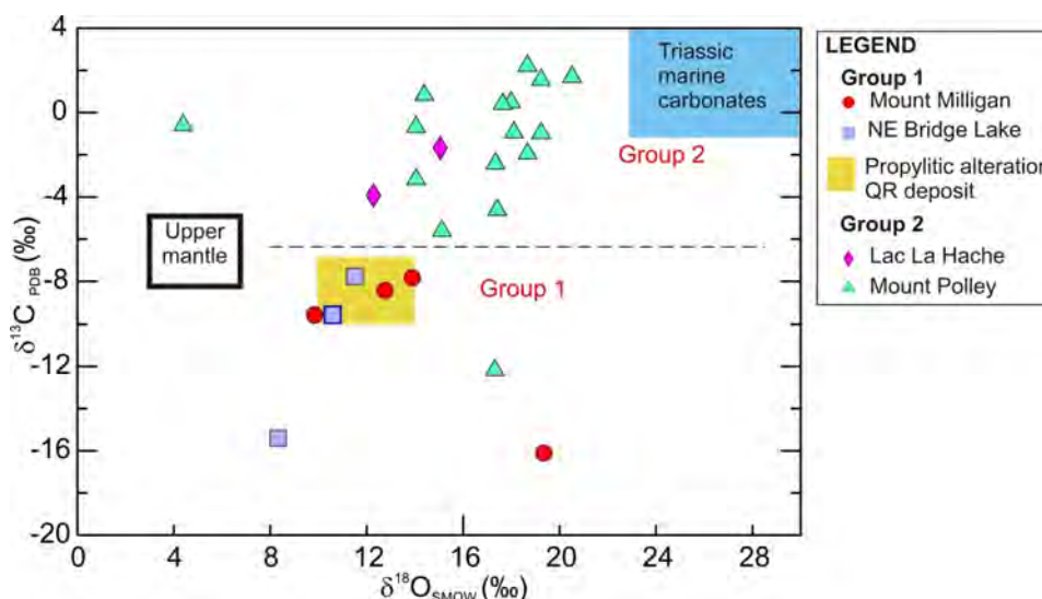
Figure 6. Plot showing the ^{18}\text{O}_{\text{SMOW}} (‰) and ^{13}\text{C}_{\text{PDB}} (‰) compositions of carbonate from basalts with propylitic alteration assemblages in the north-central part of the Quesnel terrane; fields for the Quesnel River Au deposit (Melling et al., 1990), Triassic marine carbonate rocks (Veizer et al., 1999) and upper mantle (Taylor et al., 1967) are shown for comparison.
