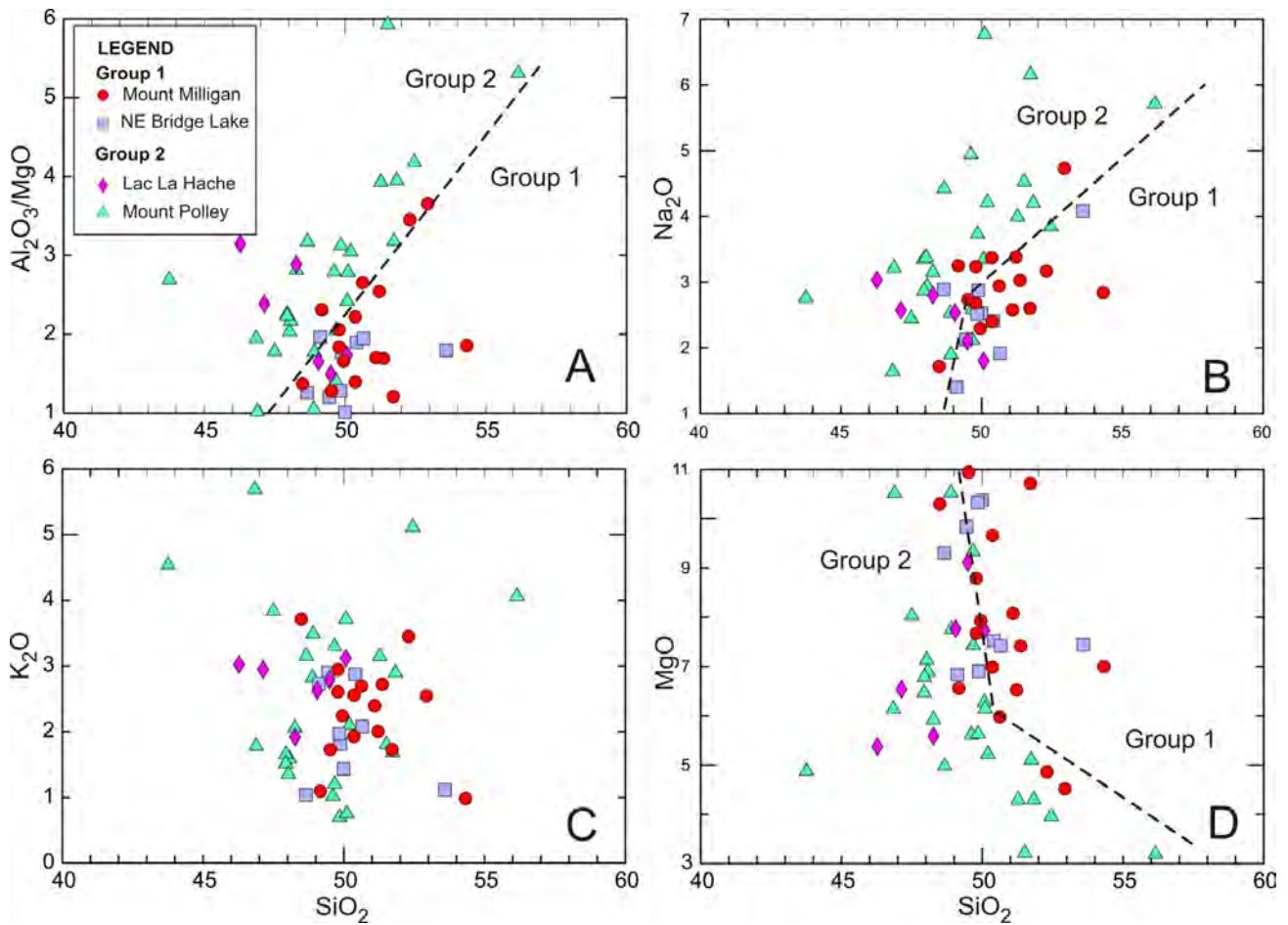
Figure 4. Harker-type diagrams for basalts from the Nicola Group. Two groups can be separated on the basis of Na and Mg content, as well as Al_2O_3/MgO ratios at given SiO_2 : group 1 includes basalts from Mount Milligan and northeast of Bridge Lake; group 2 includes basalts from the Mount Polley and Lac la Hache areas.
