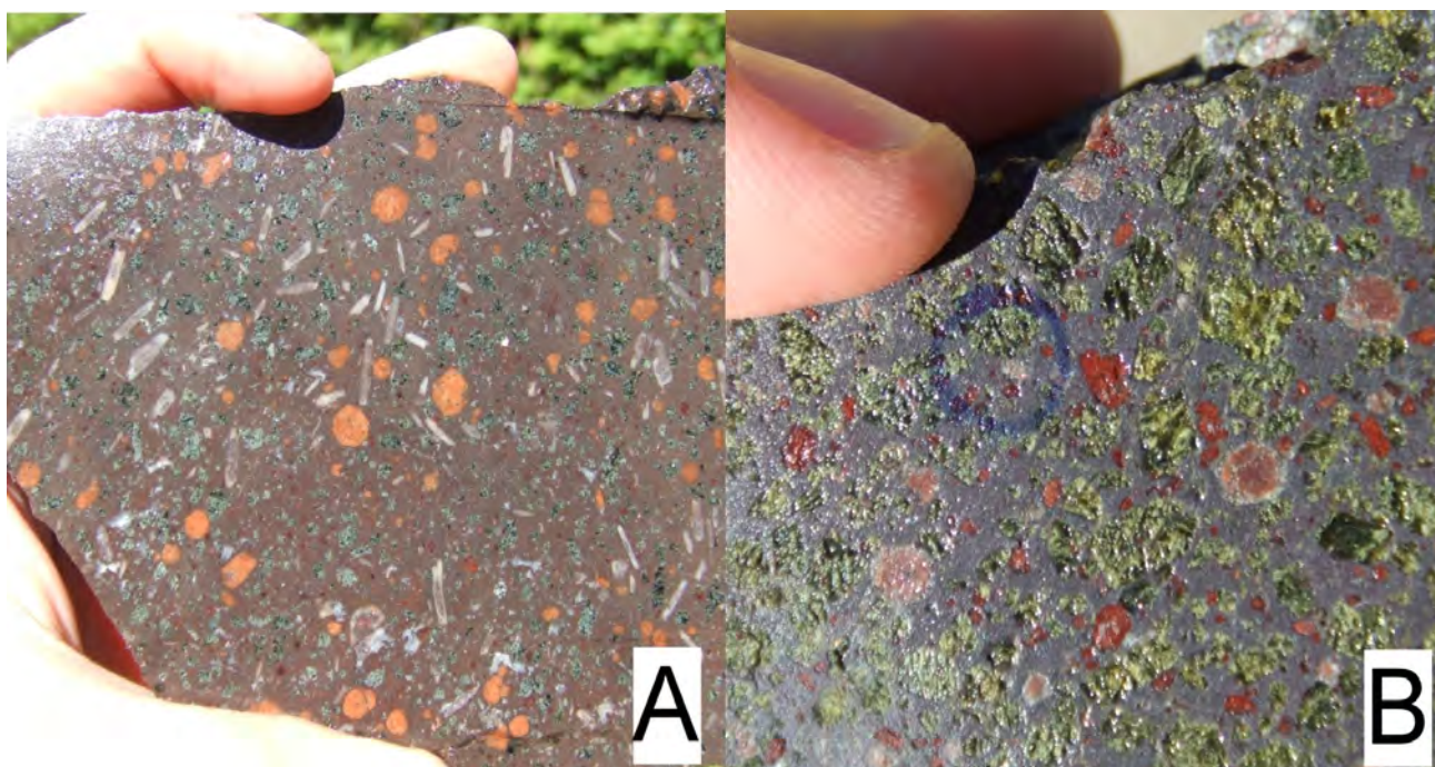
Figure 8. Analcime-bearing basalts, south-central British Columbia: A) reddish, pyroxene-plagioclase-analcime-phyric basalt in the Mount Polley area; B) pyroxene-analcime-phyric basalt of Mortimer's (1987) central belt, southern BC. The blue circle shows specks of native Cu within an analcime phenocryst.
