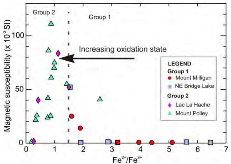
Figure 5. Plot of Fe^{2+}/Fe^{3+} versus magnetic susceptibility for weakly altered coherent basalts of the Quesnel terrane, showing the similarities between basalt samples from the Mount Milligan and northeastern Bridge Lake areas (Group 1) and the samples from the Mount Polley and Lac la Hache areas (Group 2), the latter with relatively high oxidation states and magnetic susceptibility measurements.
