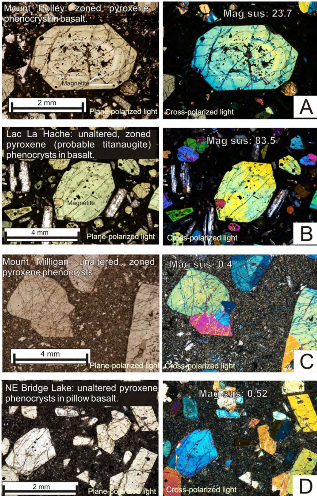
Figure 2. Unaltered zoned pyroxenes from the Nicola Group, south-central British Columbia; note that the Mount Polley (A) and Lac la Hache (B) areas contain opaque magnetite inclusions, whereas the Mount Milligan (C) and Bridge Lake (D) areas lack magnetite inclusions; magnetic susceptibility measurements for each suite are indicated.
