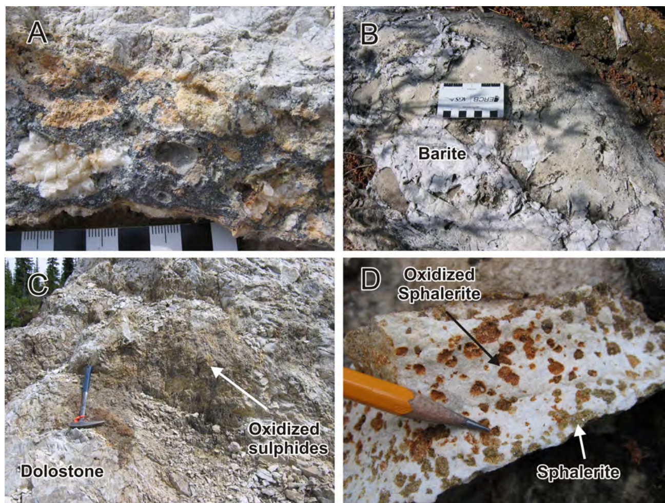
Figure 15. Gunn showing, Cariboo Zinc property, east-central British Columbia: A ) quartz–galena–nonsulphides ( \pm sphalerite) veins; B ) barite–galena–sphalerite vein crosscutting the dolostone (only barite is clearly visible in the photograph); C ) irregular replacement zones of oxidized sulphides in dolostone; D ) disseminated oxidized (orange) and fresh (yellowish) sphalerite in the fine-grained white dolostone.
