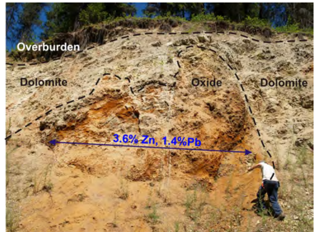
Figure 4. The main exposure at the Lomond deposit; an example of a CHNSBM deposit with an iron-rich gossan component, south-eastern British Columbia.
