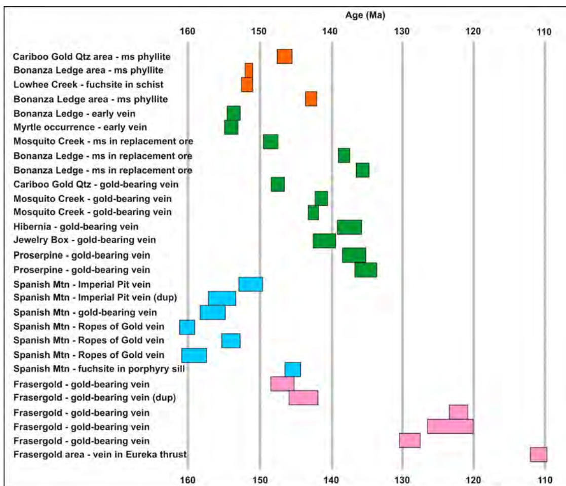
Figure 2. Compilation of all ^{40}\text{Ar}/^{39}\text{Ar} dating results from the Cariboo gold district, east-central British Columbia. Abbreviation: ms, muscovite.
