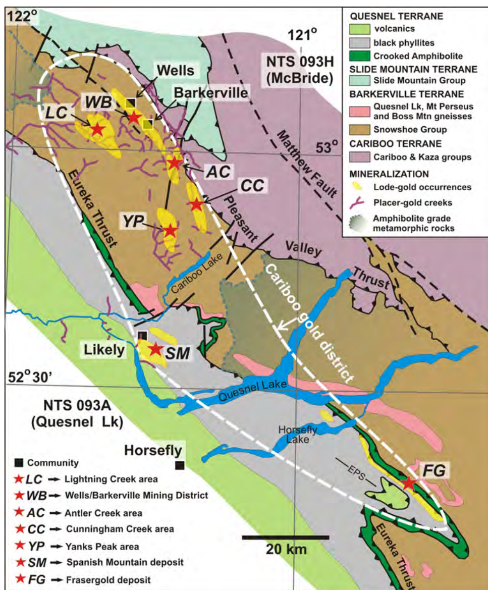
Figure 1: Regional geological setting of the Cariboo gold district, east-central British Columbia, showing principal terranes and major lithological packages. Areas of known lode-gold occurrences are shaded in yellow, and placer-gold producing creeks are indicated by thick purple lines. Principal known gold-producing areas in the Barkerville terrane are in areas of greenschist-grade metamorphism, and do not extend into amphibolite-grade domains. Abbreviation: EPS, Eureka Peak syncline.
