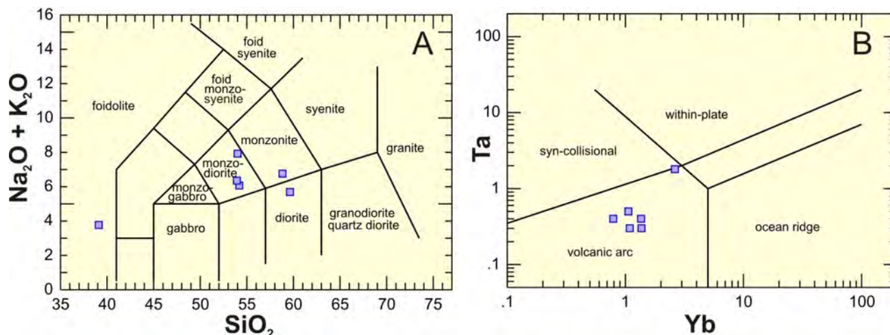
Figure 4. Compositions of Early Jurassic intrusions in the Spanish Mountain area, east-central British Columbia. Fields in A ) are from Le Bas et al. (1986) and those in B ) are from Pearce et al. (1984).
