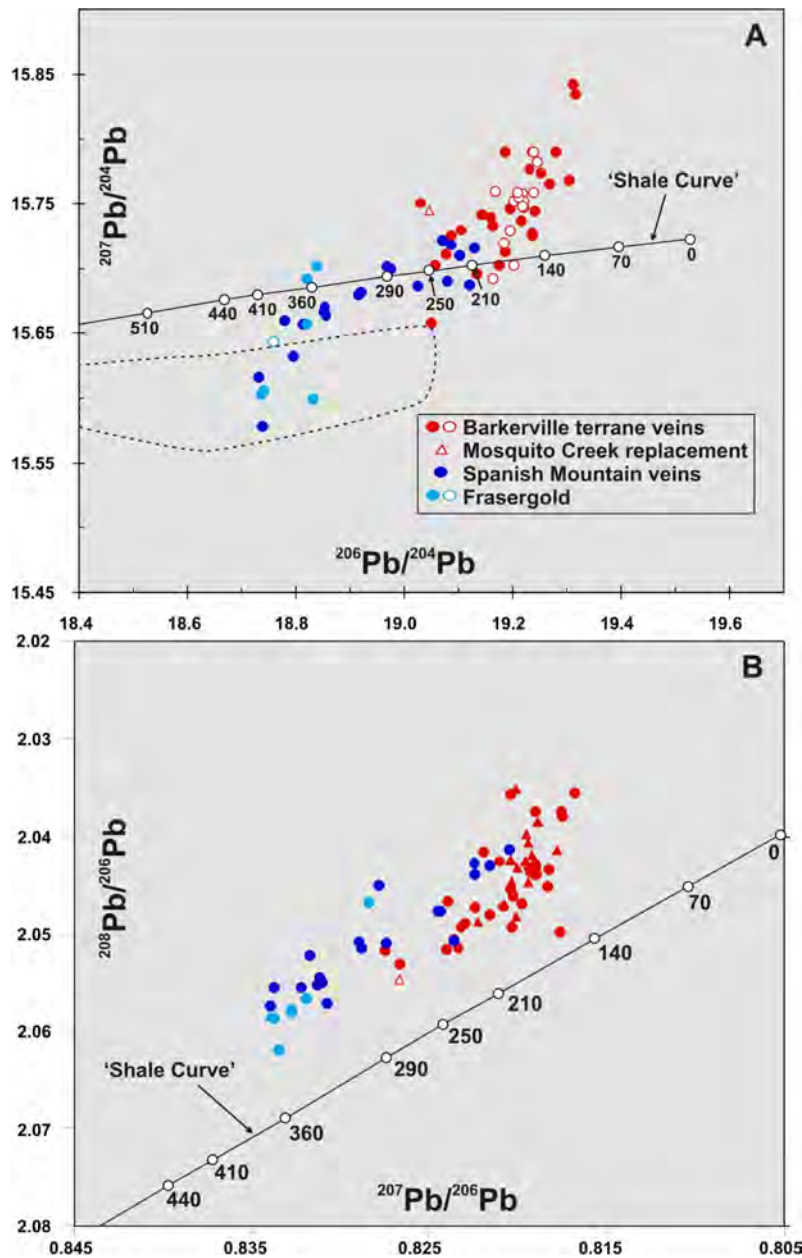
Figure 3. Lead isotopic compositions of gold-bearing veins and replacements from the Cariboo gold district, east-central British Columbia. The 'shale curve' of Godwin and Sinclair (1982) is shown for reference. The dashed outline in A ) shows the field for Pb-isotopic compositions of Nicola arc intrusive and volcanic rocks from Breitsprecher et al. (2008). Solid symbols represent analyses done as part of this study and open symbols are analyses from Godwin et al. (1988).
