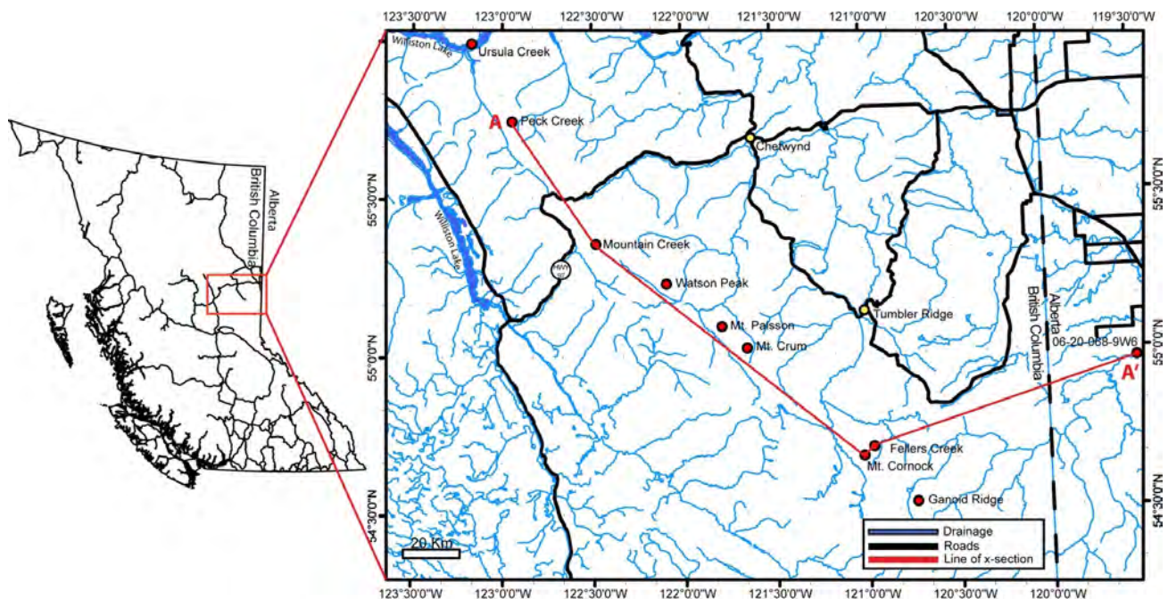
Figure 1. Study area in east-central British Columbia, showing the location of measured sections and the line of cross-section (A-A') detailed in Figure 5. Modified from Henderson et al. (2010).
