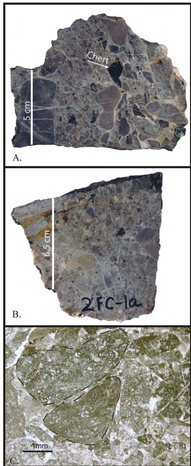
Figure 4. Photographs of cut slabs of conglomerate from Fellers Creek, east-central British Columbia: A) basal Belcourt conglomerate with chert clasts (27–27.7 m); B) second conglomerate from Fellers Creek (29.8 m); C) photomicrograph of top of second conglomerate from Fellers Creek (31.9 m), outlining subrounded carbonate clasts. All measurements are from the base of the section.
