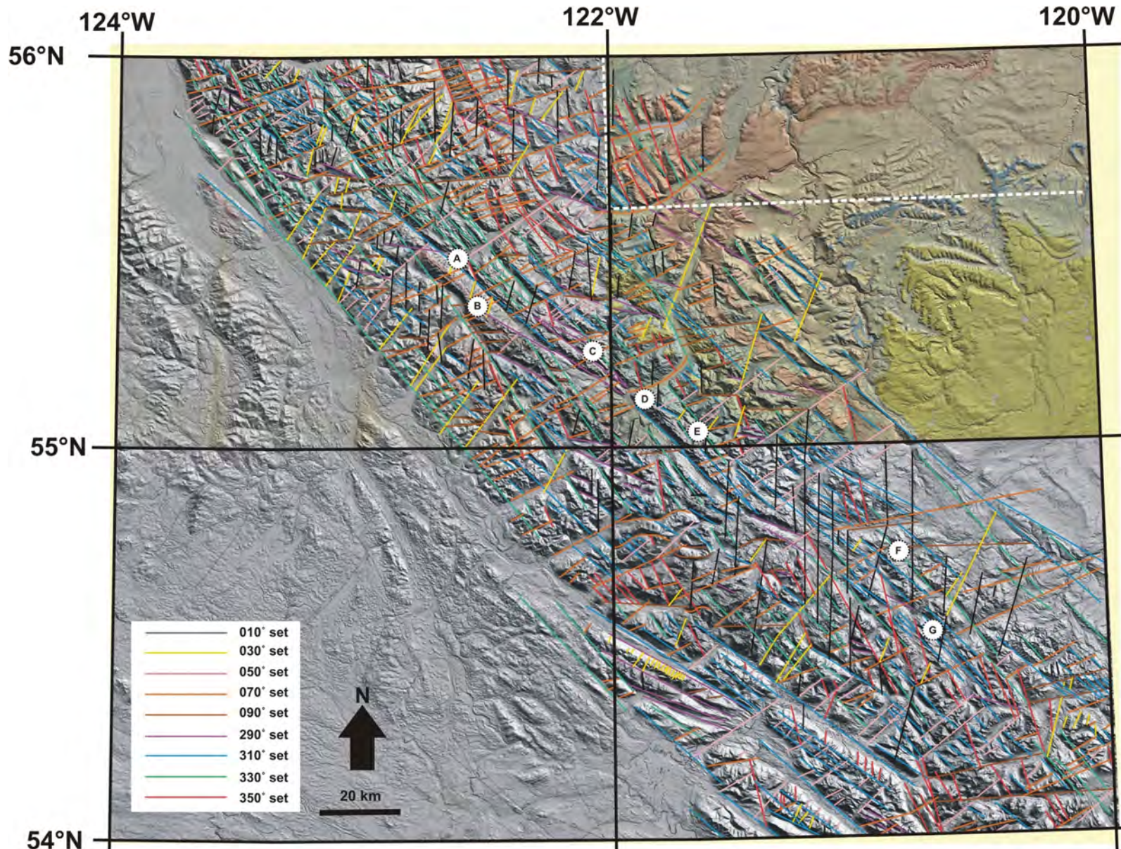
Figure 6. Digital elevation model (DEM; data from GeoBase) of the study area, illustrating macro-scale lineament orientations: A) Solitude Mountain, B) Mountain Creek, C) Watson Peak, D) Mount Palsson, E) Mount Crum, F) Fellers Creek, and G) Ganoid Ridge. Dashed white box denotes the Fort St. John block, an extension of Alberta townships and ranges into British Columbia between 55.65 and 56.65 N and 120 and 122 E (map adapted from Stott et al., 1983; McMechan and Thompson, 1989, 1994).
