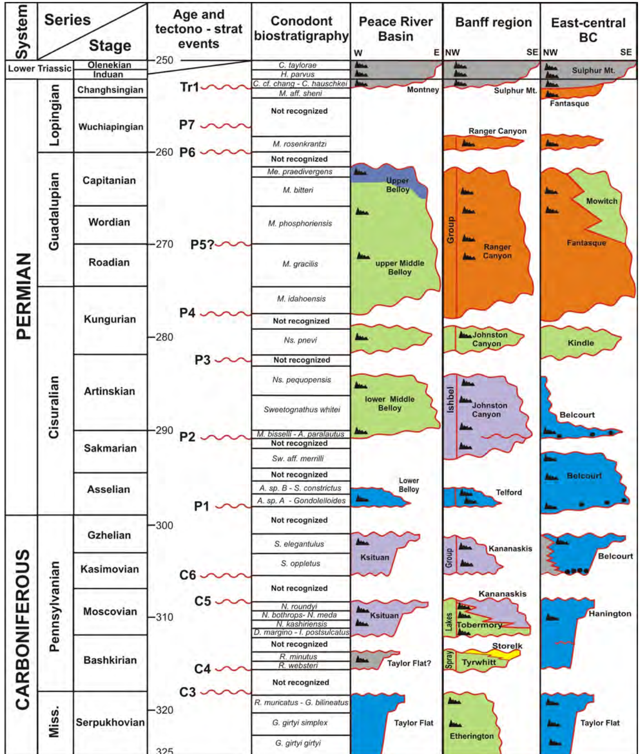
Figure 2. Stratigraphy and tectonostratigraphic sequences of east-central British Columbia correlated to the Peace River Basin of west-central Alberta and northeastern British Columbia, and the southwestern Alberta Rockies ('Banff region'). Tectonostratigraphic sequences are from Snyder et al. (2002), Trexler et al. (2004) and Henderson et al. (2010). Stratigraphy is modified from Henderson et al. (2010). Conodont symbols indicate control points. Colours represent primary lithology, including limestone (blue), dolostone (purple), chert (orange), quartz arenite (yellow), bioturbated and bioclastic sandstone (green) and silty shale (grey). Abbreviations: C, Carboniferous; P, Permian.
