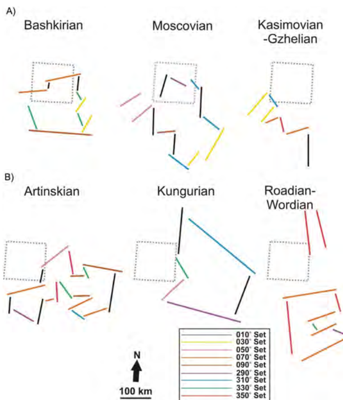
Figure 7. Schematic diagram illustrating the dominant sub-basin orientations (see legend) in the A) Pennsylvanian, and B) Permian. The dashed grey boxes denote the present-day position of the Fort St. John block. Adapted from Dunn (2003) and Dean (2010).
