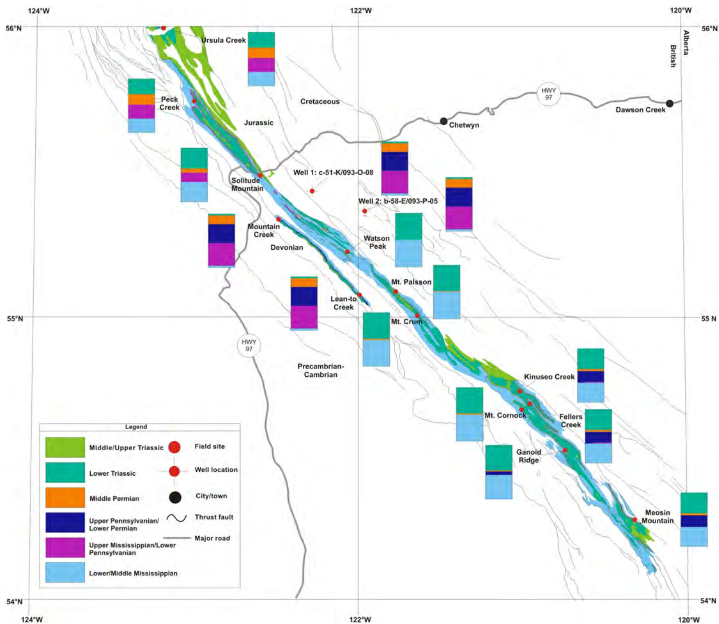
Figure 9. Geology of the east-central British Columbia study area, showing schematic summary columns of strata present at each outcrop. Note missing Early Permian strata at Watson Peak, Mount Palsson, Mount Crum and Mount Cornock, defining a southeast-trending linear paleo-high.
