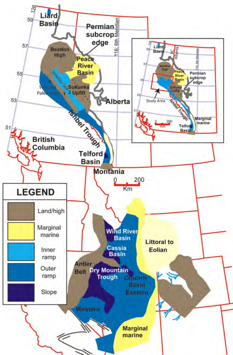
Figure 3. Simplified late Sakmarian paleogeography of western North America, showing significant tectonic elements and the interpreted location and configuration of the newly defined (this paper) western paleo-high, extending south from the Beaton High. Numbered features: 1, Mount Cornock; 2, Fellers Creek; 3, Mountain Creek. Paleogeographic features associated with the Antler Orogeny in the western United States are also labelled. Inset in upper right is of known and published simplified paleogeography in west-central Alberta, with study area outlined in red. Modified from Henderson et al. (2002).
