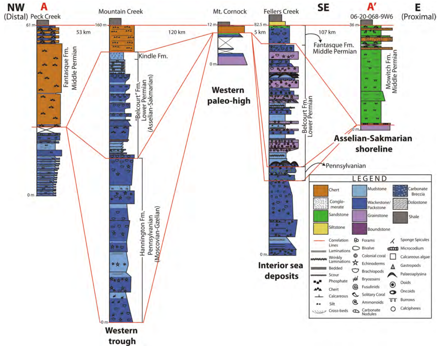
Figure 5. Cross-section A–A' (see Figure 1 for location), showing stratigraphic relationships between outcrops, rock types and formations. The western paleo-high and interior sea shown in Figure 3 are also labelled. Stratigraphic units include, in ascending order, Mississippian (below the lowest red line), Pennsylvanian Hannington Formation, Pennsylvanian–Early Permian Belcourt Formation, Early Permian Kindle Formation and middle Permian Fantasque Formation. The stratigraphic datum is the base of the Triassic Sulphur Mountain Formation.
