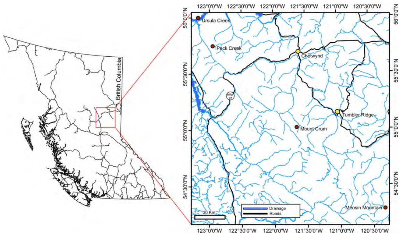
Figure 1. Study area in east-central British Columbia, showing the locations of sections (using NAD 83): Meosin Mountain, 54.28616 N, 120.32557 W; Mount Crum, 55.02541 N, 121.65057 W; Peck Creek, 55.75045 N, 122.95348 W; and Ursula Creek, 55.99312 N, 123.17426 W.
