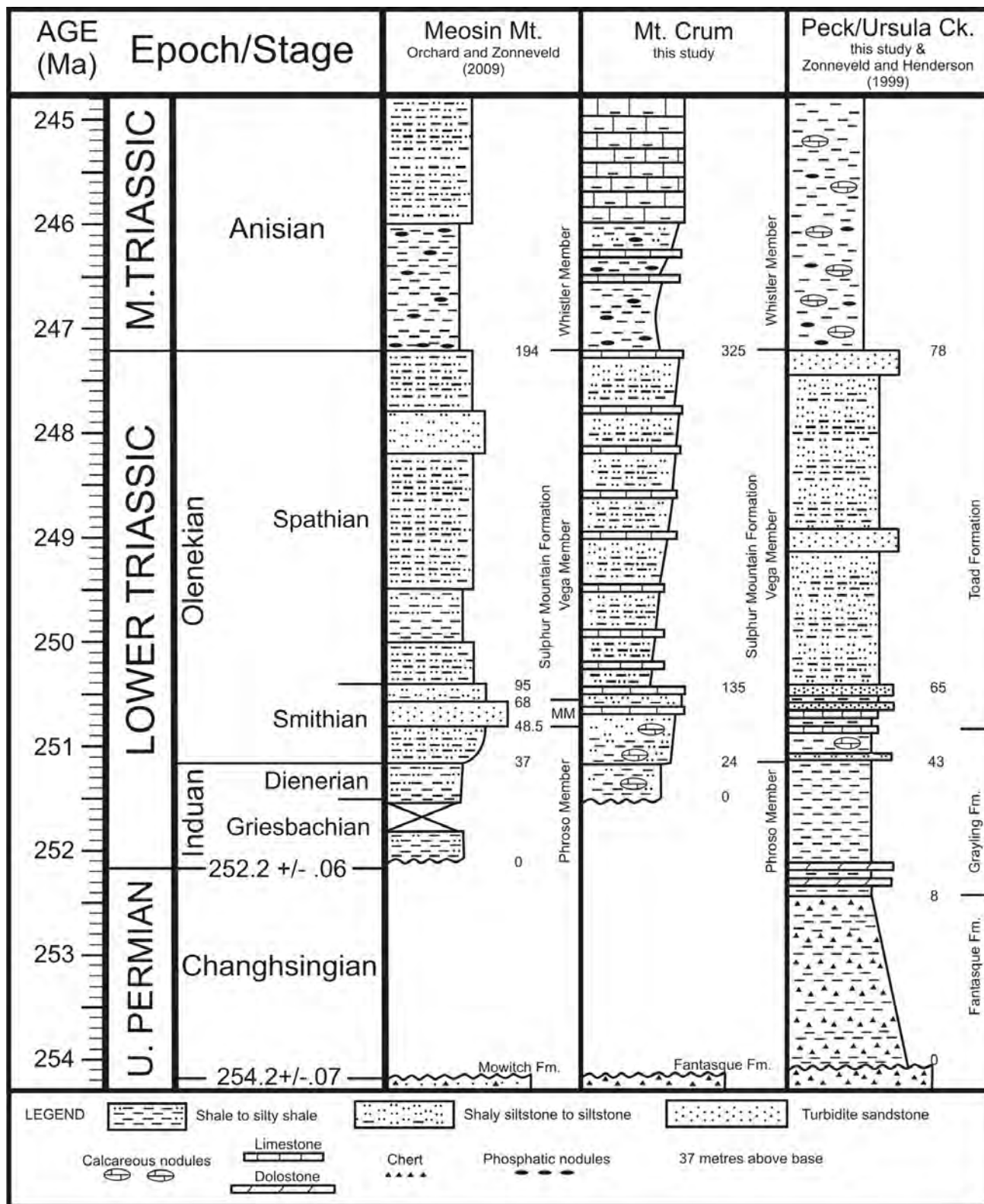
Figure 3. Lithology for Meosin Mountain, Mount Crum and the Peck Creek and Ursula Creek composite, east-central British Columbia. Stratigraphic units are arranged according to time, and measurements above base in metres are provided at key points. MM, Meosin Mountain Member.
