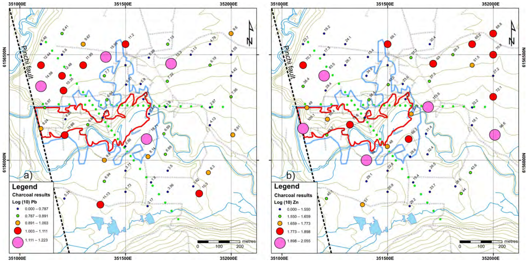
Figure 8. Analytical results for charcoal samples, north-central British Columbia: a) Pb and b) Zn. Scaled symbols represent log (10) transformed values; raw values (in ppm) are plotted next to each symbol. Surface projection of mineralized zone (Central zone) is outlined in red for 0.6% Cu equivalent and blue for 0.2% Cu equivalent. Green dots indicate 2009 transects.
