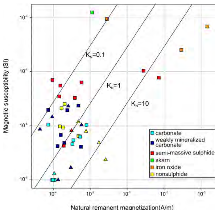
Figure 5. Plot of magnetic remanence versus magnetic susceptibility, with lines of equal Koenigsberger ratio ( K_N ) indicated, samples from Salmo and Quesnel Lake camps, south-central British Columbia. Note that nearly half the samples have K_N > 1 . Salmo camp samples are plotted as squares while Quesnel Lake samples are plotted as triangles.
