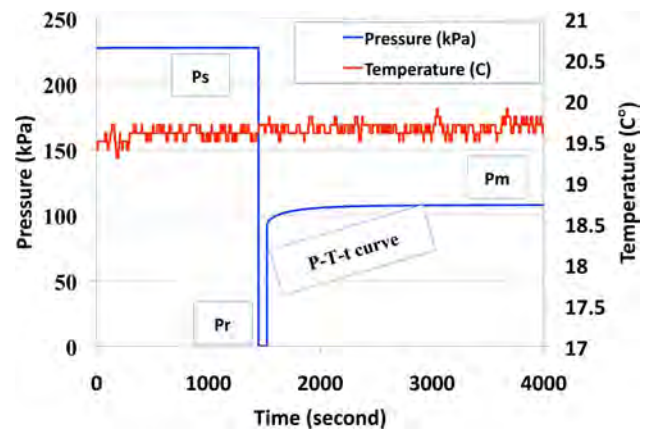
Figure 3. Typical pressure and temperature data of porosity and permeability analyses carried out on core from the study area in northeastern British Columbia (after Cui et al., 2010). Abbreviations: initial equilibrium pressure in sample cell, P_s ; reference cell pressure, P_r ; final equilibrium pressure, P_m .
