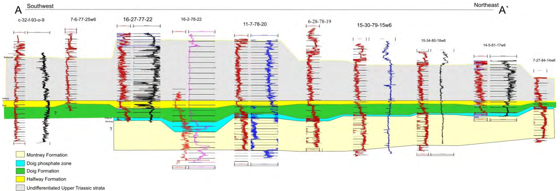
Figure 5: Cross-section A–A' showing the stratal geometries of the Triassic sediments sampled from wells located along the depositional dip in the study area, in northeastern British Columbia. Geophysical logs include gamma ray (red curve), bulk density (black curve), sonic density (blue curve) and gas content (magenta curve).
