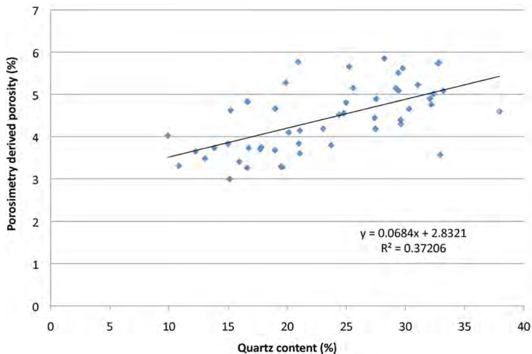
Figure 8. Plot showing positive trend between quartz content and porosity-derived porosity for well 16 2-78-22 in northeastern British Columbia.
