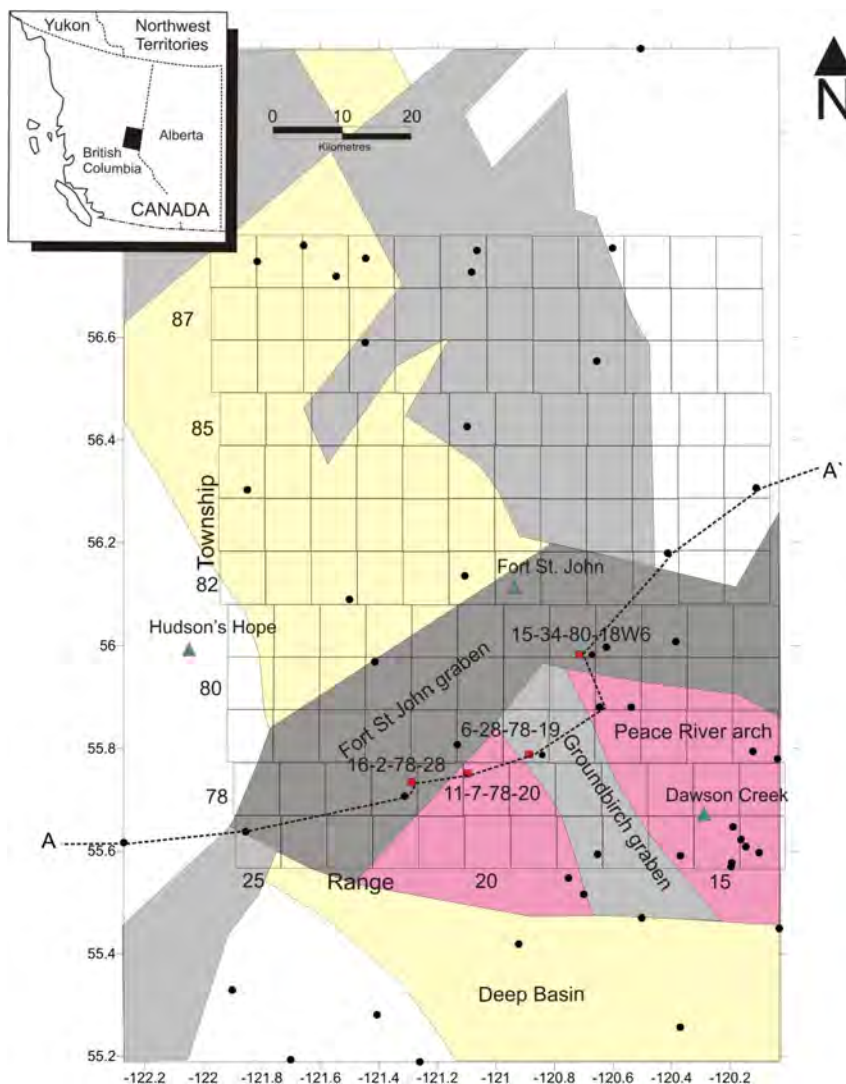
Figure 4. Index map showing the location of the Doig and Montney formations, and the location of cross-section A–A' in northeastern British Columbia (Figure 5). Red squares represent wells that are sampled for this project and green triangles, the locations of cities and towns. The structural elements for the area are modified from Berger et al. (2008), with both the darker and lighter grey areas representing the Fort St. John and Groundbirch graben system. Black circles represent the locations of wells used in this study to date.
