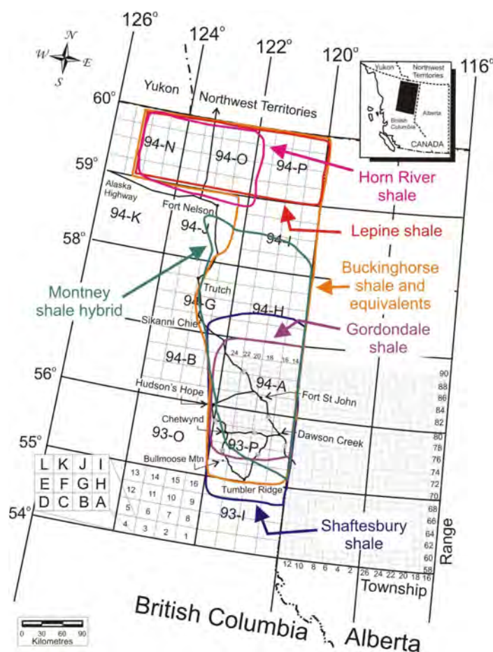
Figure 1. Approximate boundaries or limits of available core for the major potential gas-shale reservoirs in northeastern British Columbia (modified from Mossop and Shetsen, 1994).
