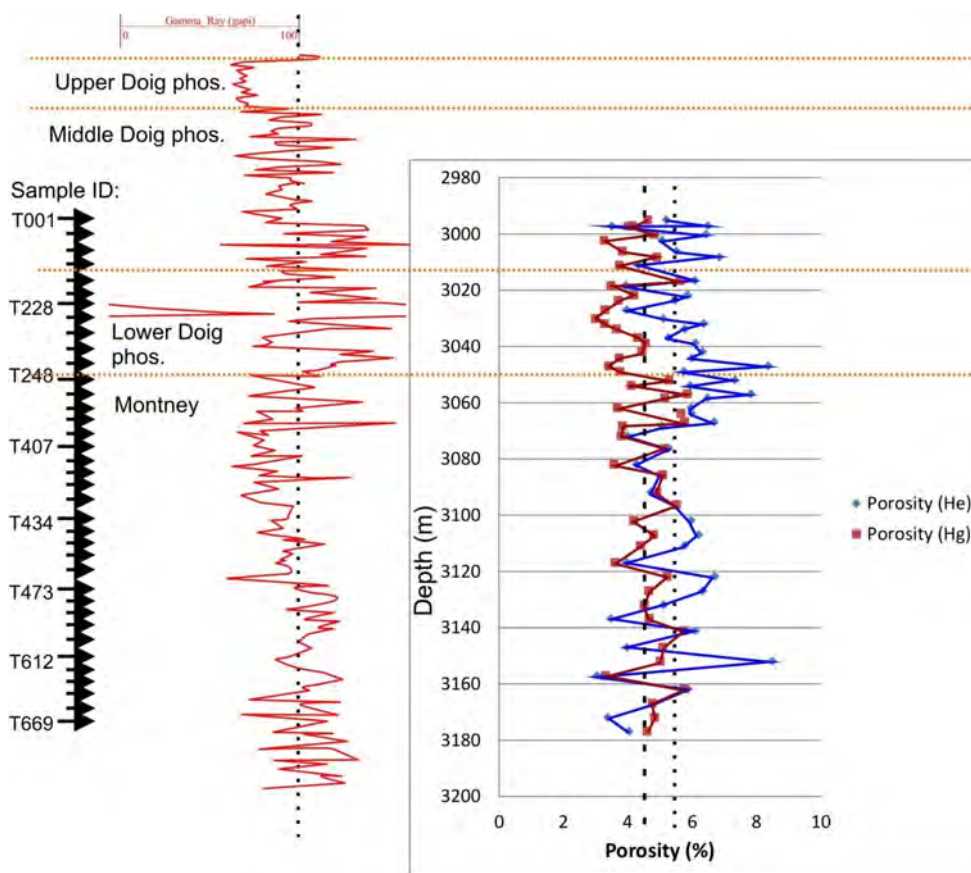
Figure 7. Gamma-ray curve (left) and pycnometry- and porosimetry-derived porosity profile (porosity variation with depth) for well 16-2-78-22 in northeastern British Columbia. Dashed line represents the porosimetry (Hg)-derived porosity and the dotted line, the pycnometry (He)-derived porosity. Black arrows indicate sampling locations. Abbreviations: helium, He; mercury, Hg.
