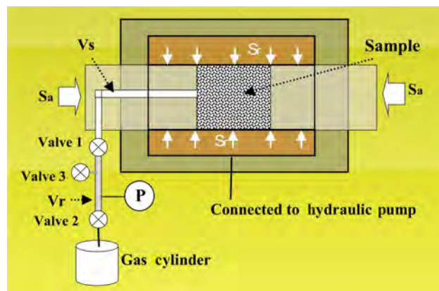
Figure 2. Connectional diagram of instrument designed to measure effective gas porosity of core plugs from study area in north-eastern British Columbia. Abbreviations: pressure transducer, P; axial stress, S_a ; reference cell void volume, V_r ; sample cell void volume, V_s .
