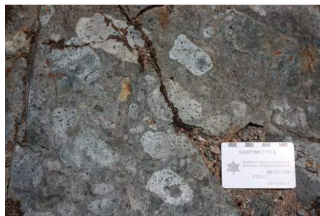
Figure 3. Coarse-grained epiclastic volcanogenic rocks from the Copper River area, British Columbia. Clasts are predominantly porphyritic andesite and dacite.
