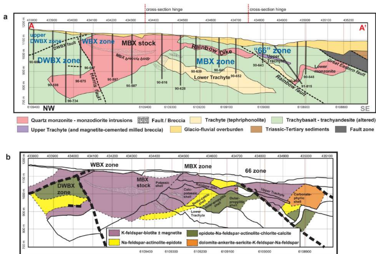
Figure 3: Profile view of the Mount Milligan alkalic porphyry Cu-Au deposit along the hinged cross-section showing a) interpreted geology, major structures, four ore-zone divisions of the MBX Main deposit (DWBX, WBX, MBX, and 66), and locations of the drillholes investigated (original lithology provided by Placer Dome Inc.); b) distribution of alteration assemblages superposed on the geology.
