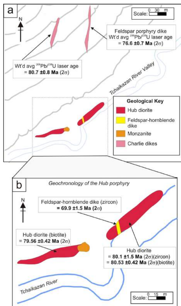
Figure 3. Maps of the Hub porphyry deposit and surrounding Charlie dikes showing: a) geological and b) geochronological data.
