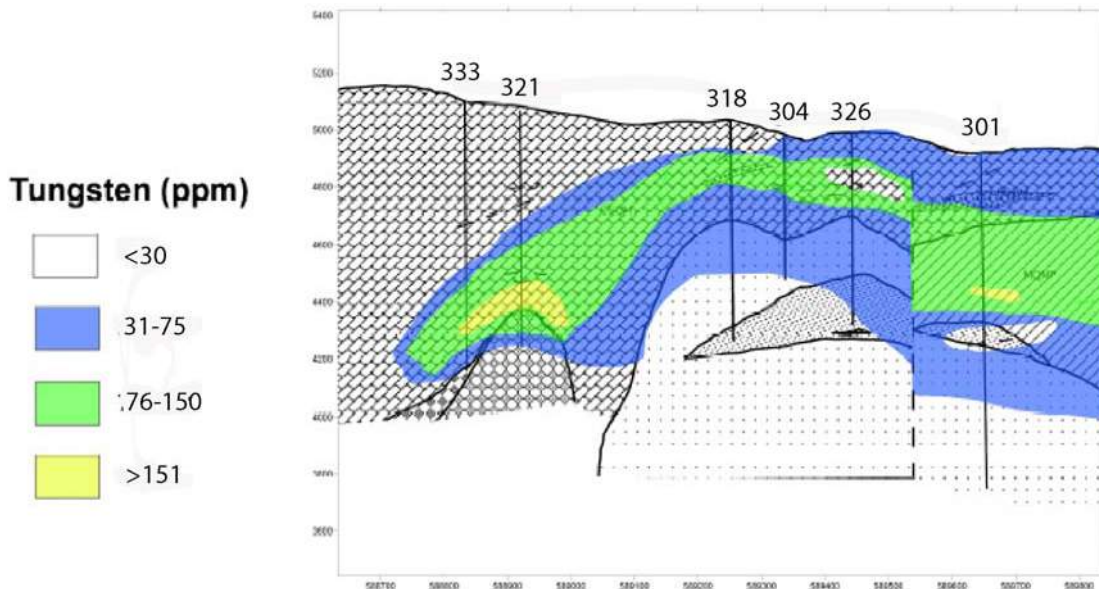
Figure 9. Cross section A-A', showing geology (rock type occurrences, faults and some silicification zones) in black and white, and W (in ppm) contoured against the black-and-white background; key as in Figure 7.
