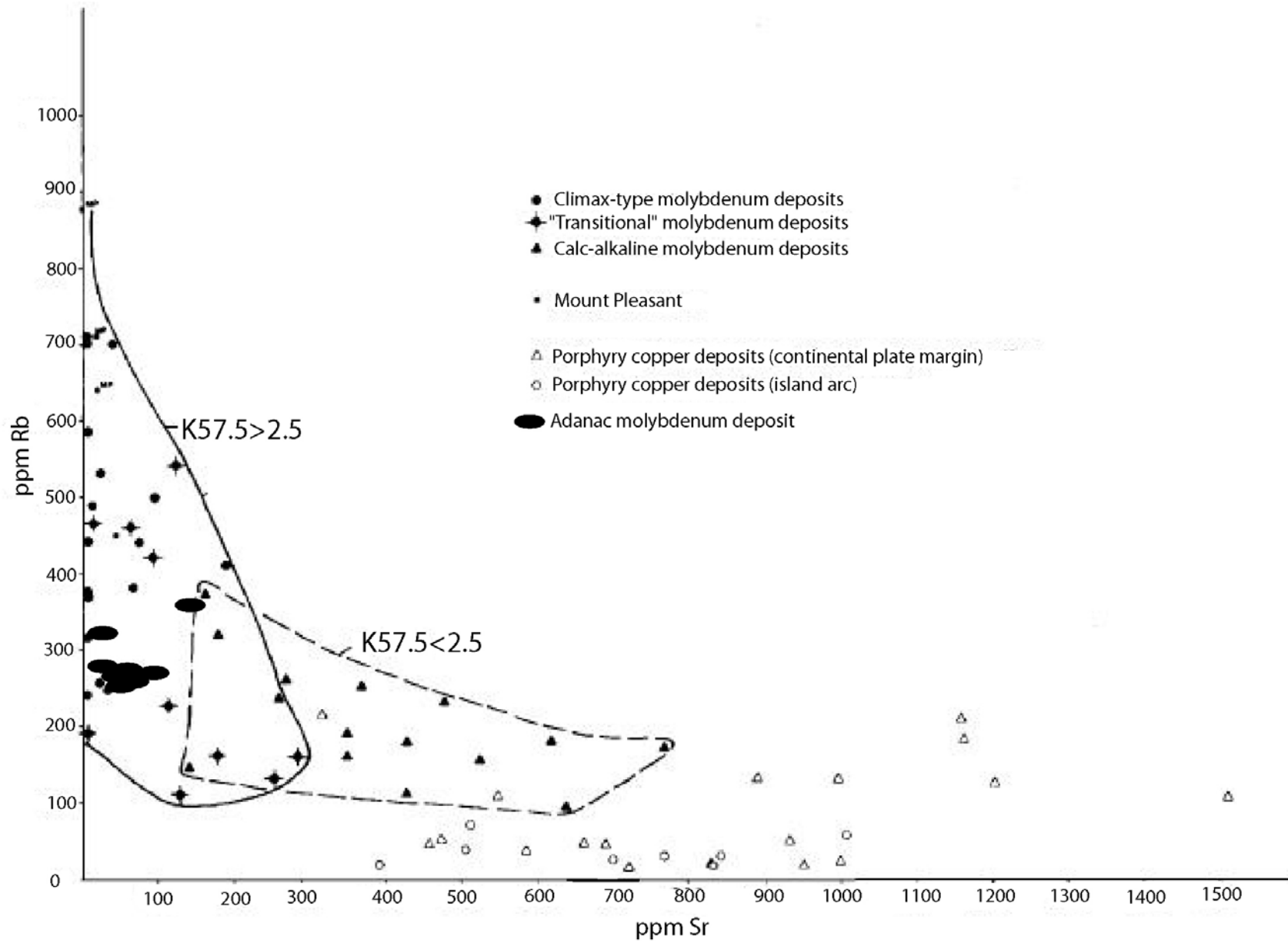
Figure 6. Graph showing Rb and Sr values for various types of porphyry deposits, including Cu porphyry and a W-Mo porphyry (Mt. Pleasant). The K_{2O_{57.5}} value fields are superimposed on the graph. As their K_{2O_{57.5}} value would indicate, rocks at Adanac fall within the field of climax-type deposits.
