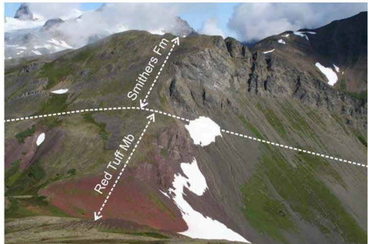
Figure 4. Stratigraphic contact between the Red Tuff Member and the Smithers Formation at Ashman Ridge.
