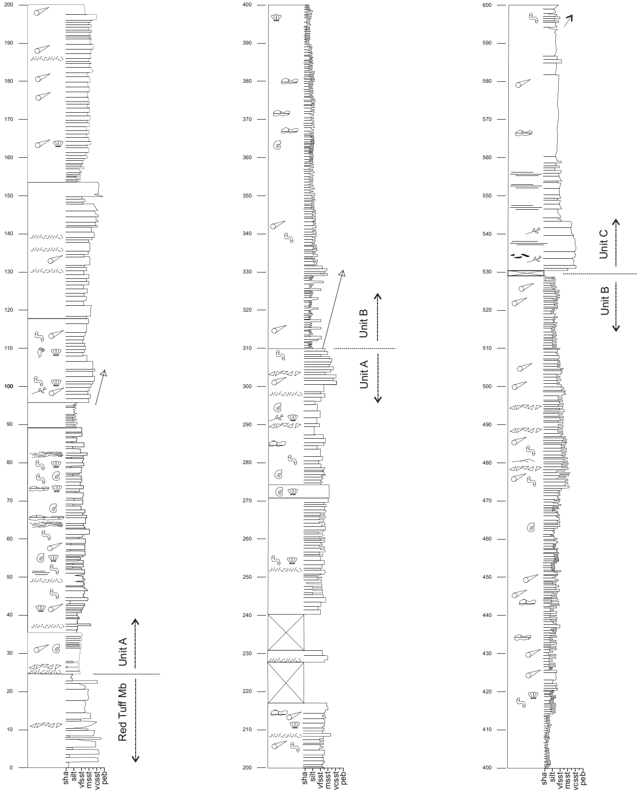
Figure 5. Detailed stratigraphic section at Ashman Ridge, showing the different units identified in this study.
