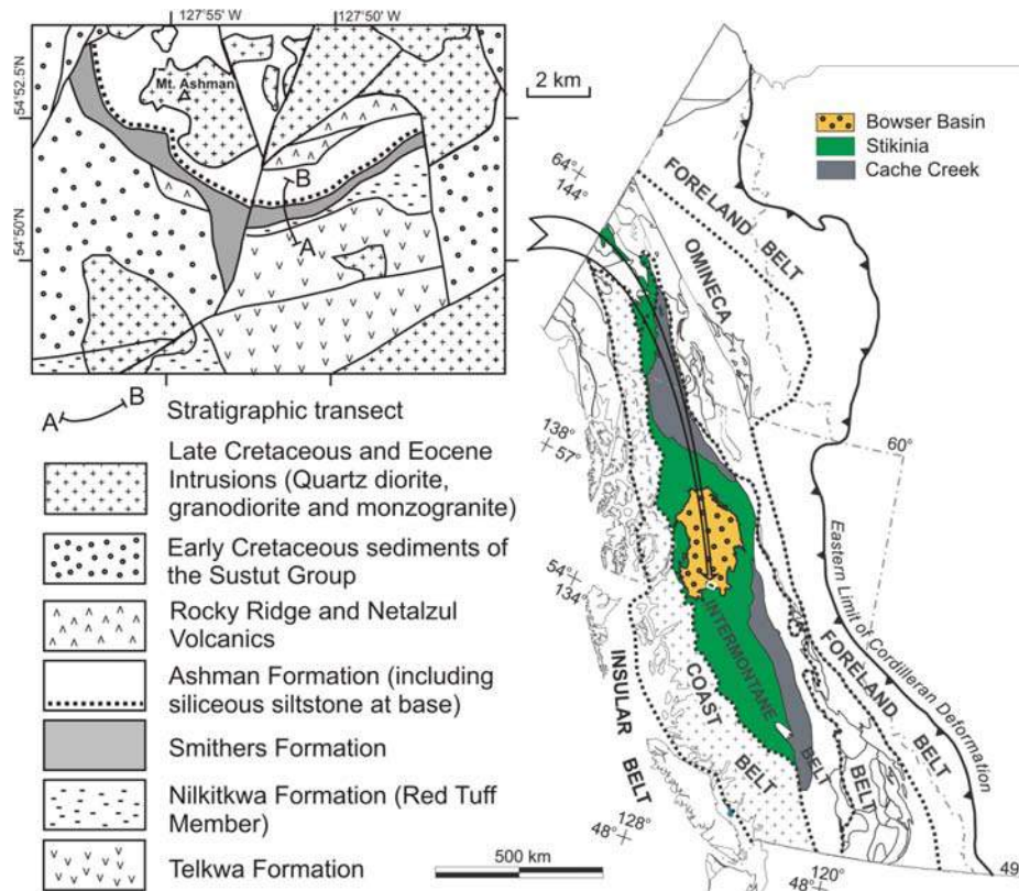
Figure 1. Simplified geology of the Ashman Ridge area, showing the location of the stratigraphic transect described in this study. Right side of the figure shows the location of the Bowser Basin in relation to principal tectonic belts of the Canadian Cordilleran Orogen ( modified from Tipper and Richards, 1976; Evenchick and Thorkelson, 2005).
