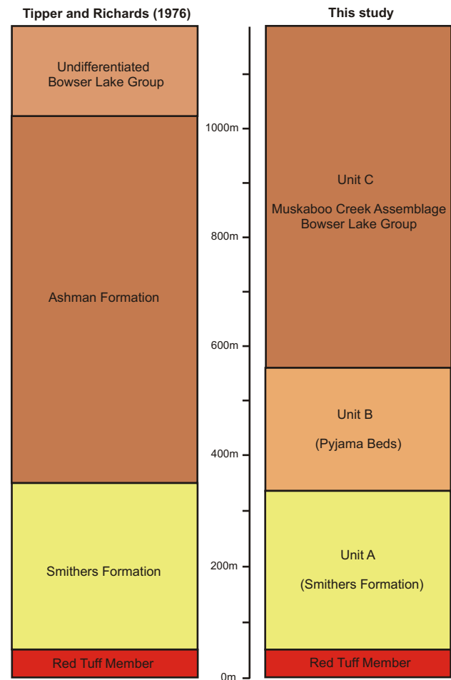
Figure 9. Stratigraphic correlations between the detailed section of this study and the original type section of the Ashman Formation (Tipper and Richards, 1976).
